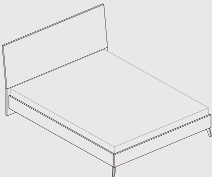
Q.S./160 L 168 W 217 H 117 cm. 180 L 188 W 217 H 117 cm. K.S. L 203 W 217 H 117 cm.
